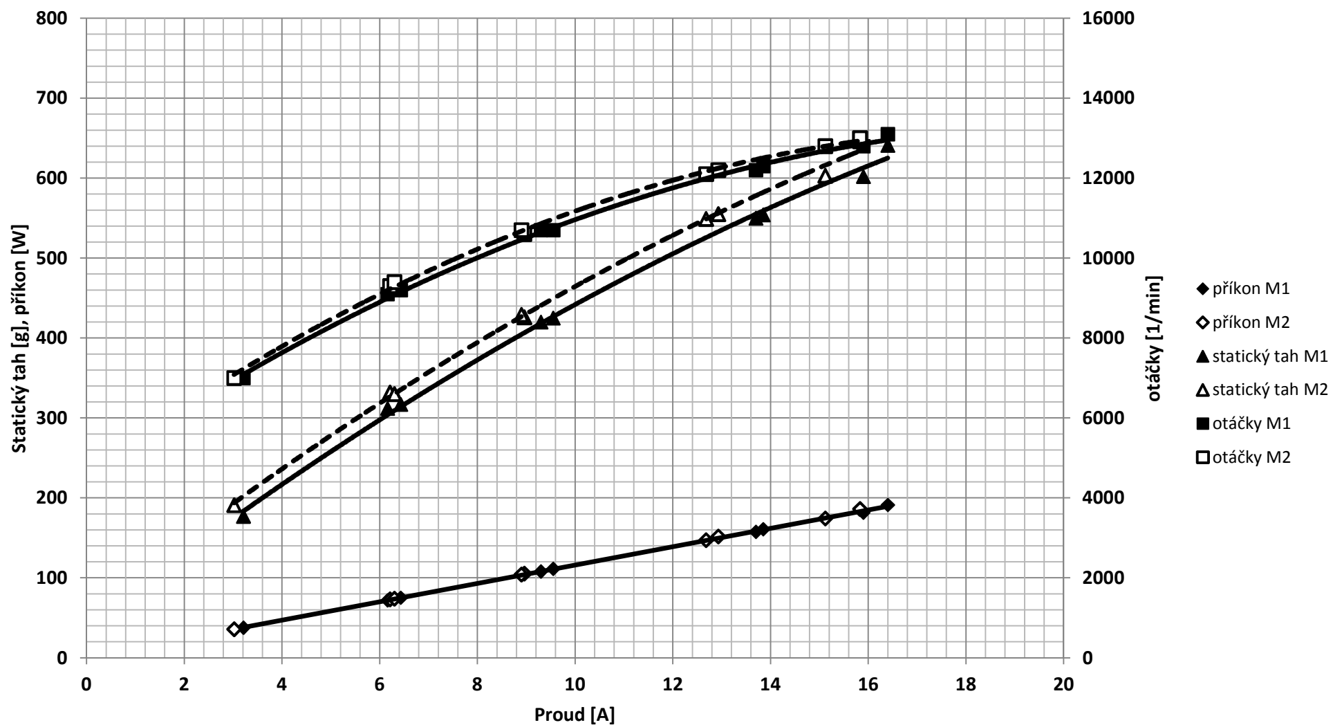
Turnigy 2836-1000 & Turnigy Plush 30A & APC 7x5" @ 11.6V, timing: middle
